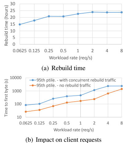
Figure 7: Scheduler performance.
