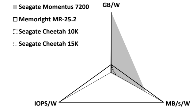
Figure 7. Device capabilities normalized by power consumption.
